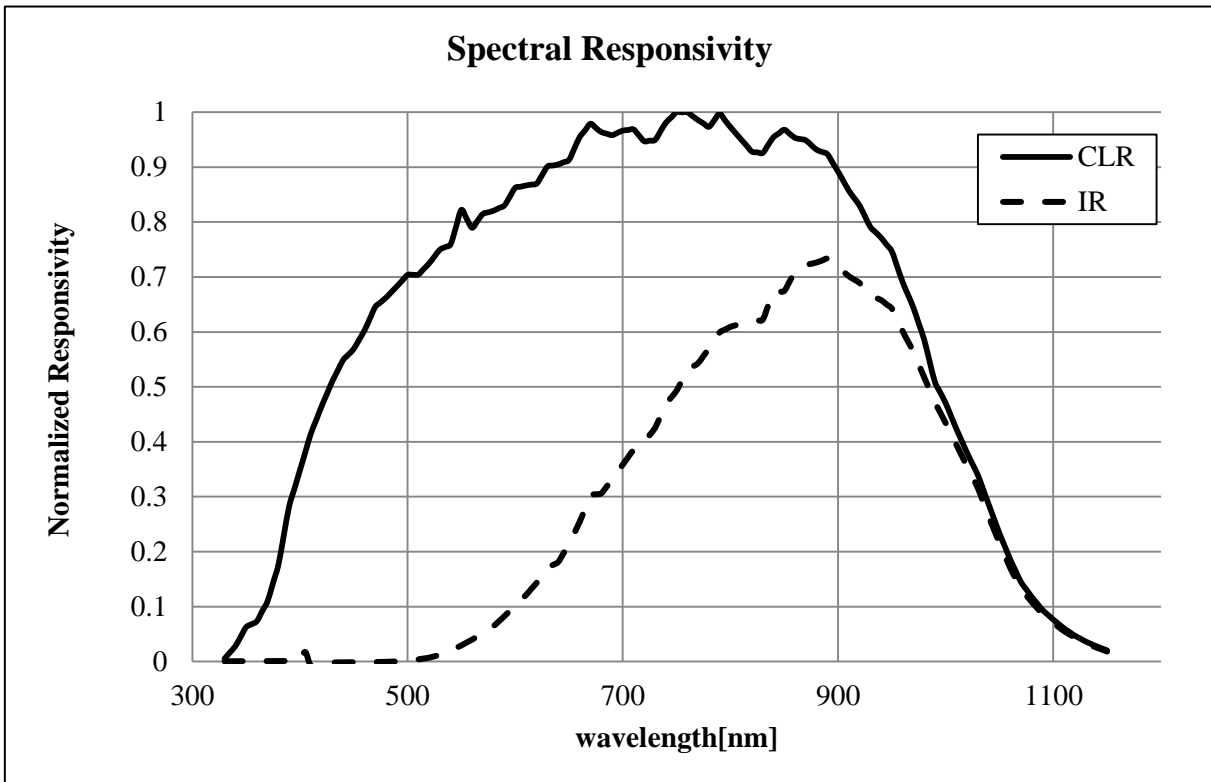
Fig.20 Spectral Responsivity
