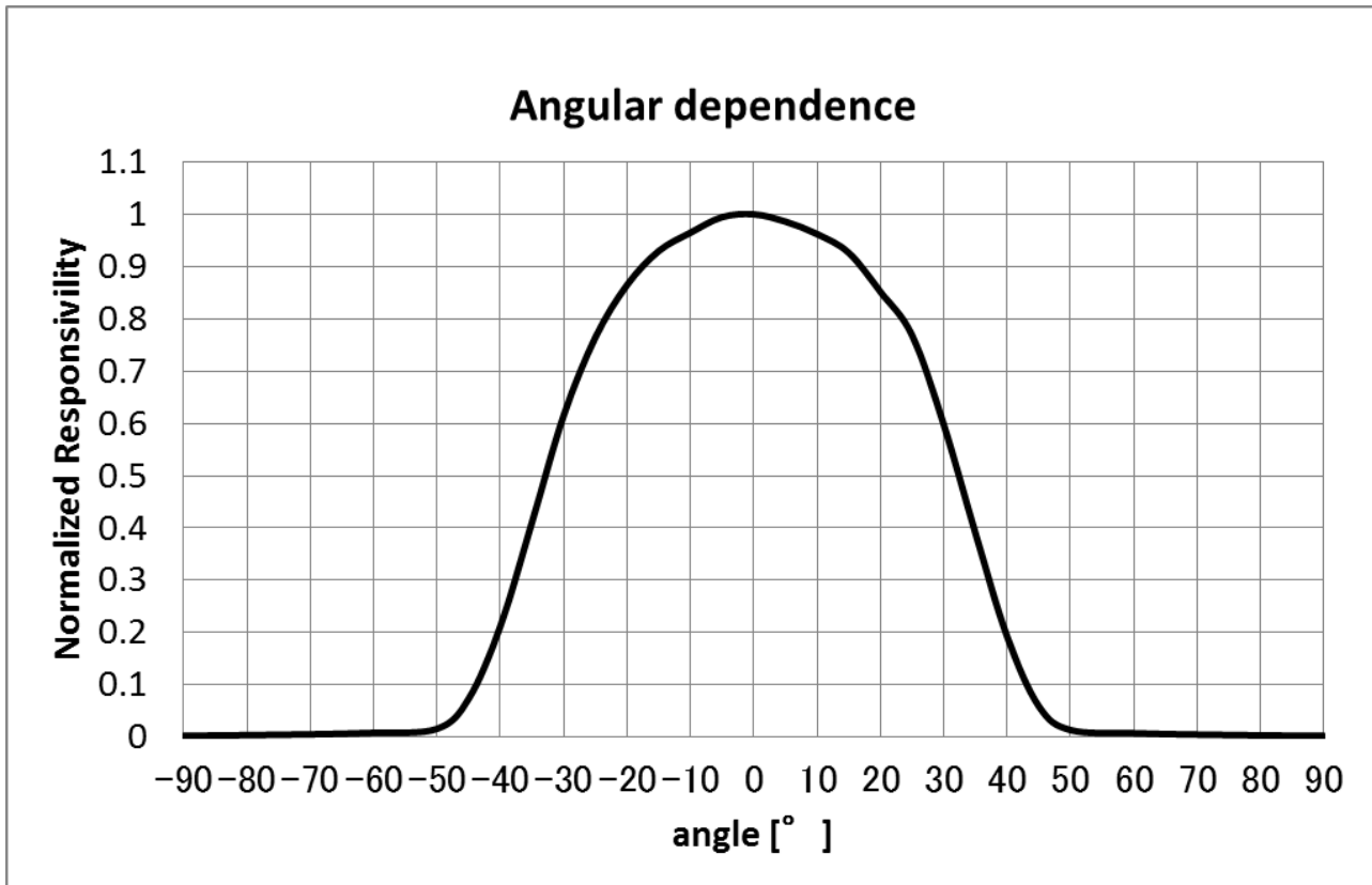
Fig.22 Angular dependence
