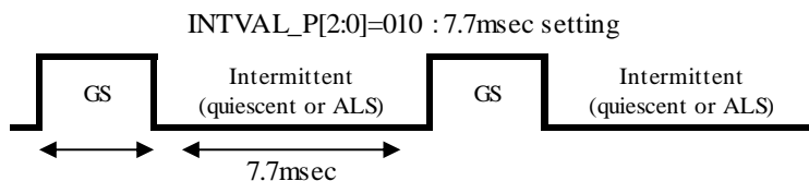
Fig.13 Intermittent operating
