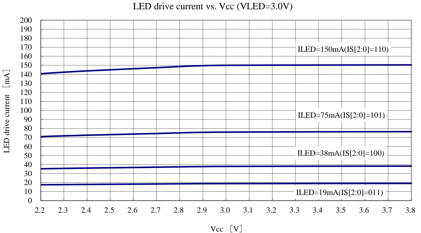
Fig.19 LED drive peak current vs. Vcc
