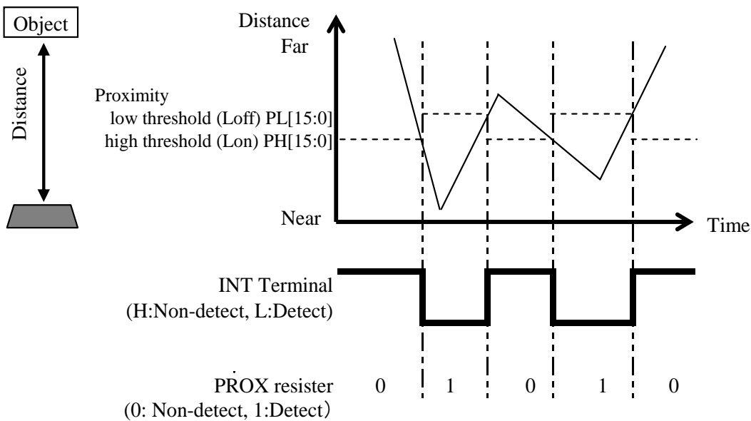
Fig.9 Detection result output mode
