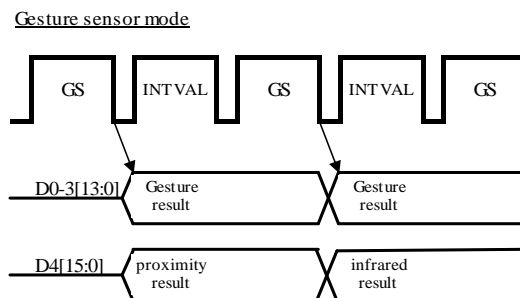
Fig.6 Output results for GS mode
