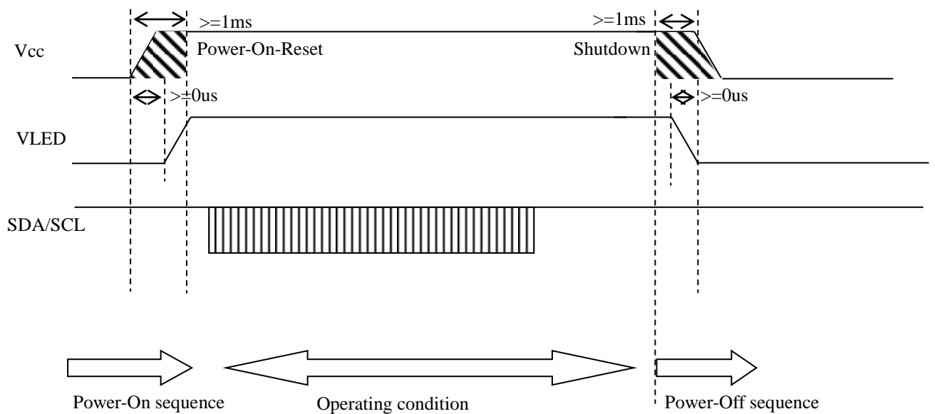
Fig.16 Power-On and Power-Off
