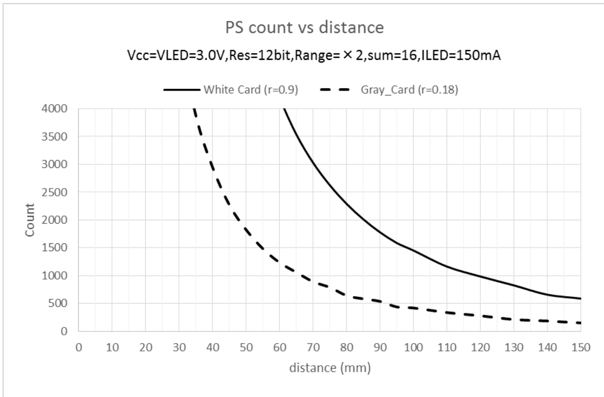
Fig.21 Sensor output counts vs. distance
