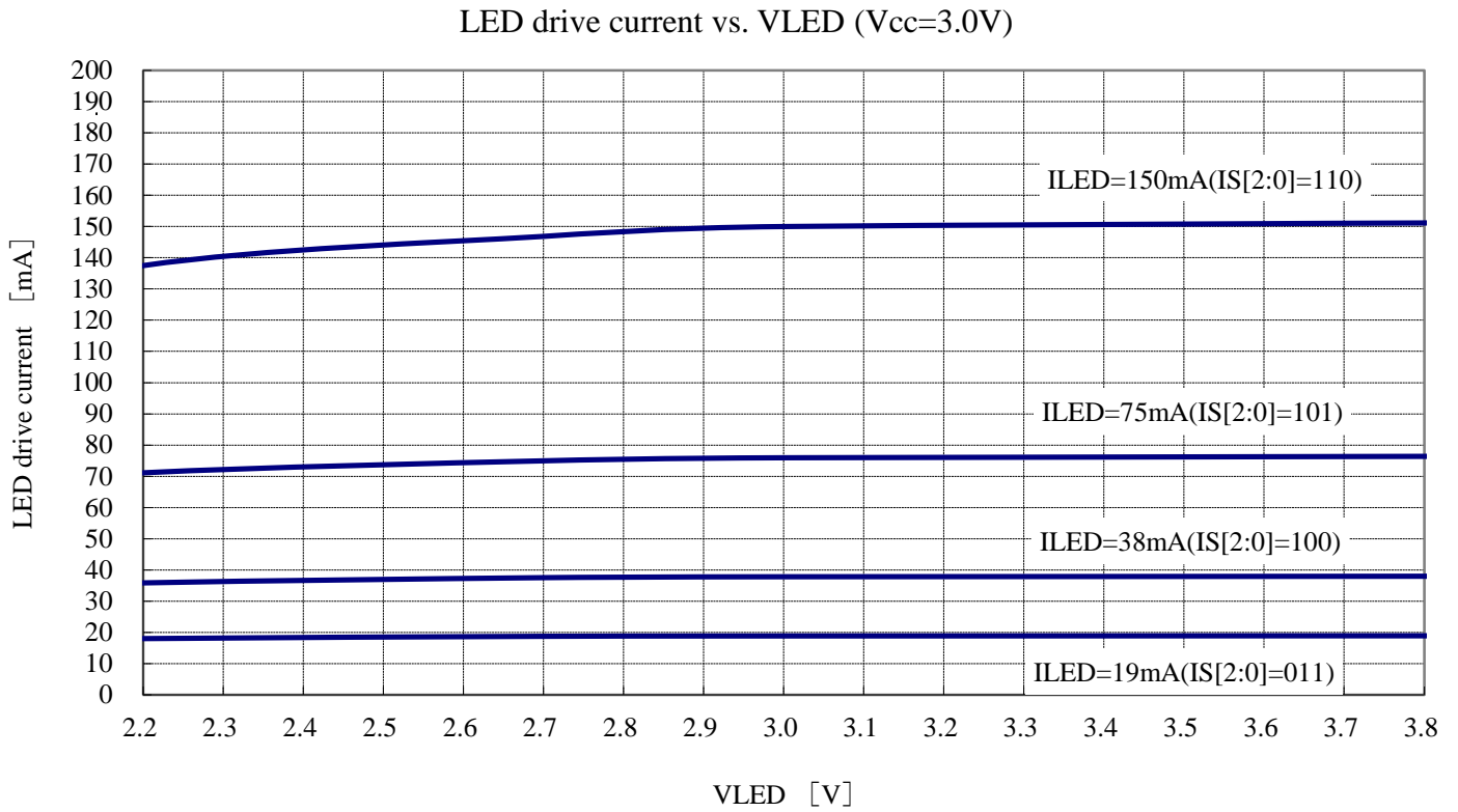
Fig.18 LED drive peak current vs. VLED
